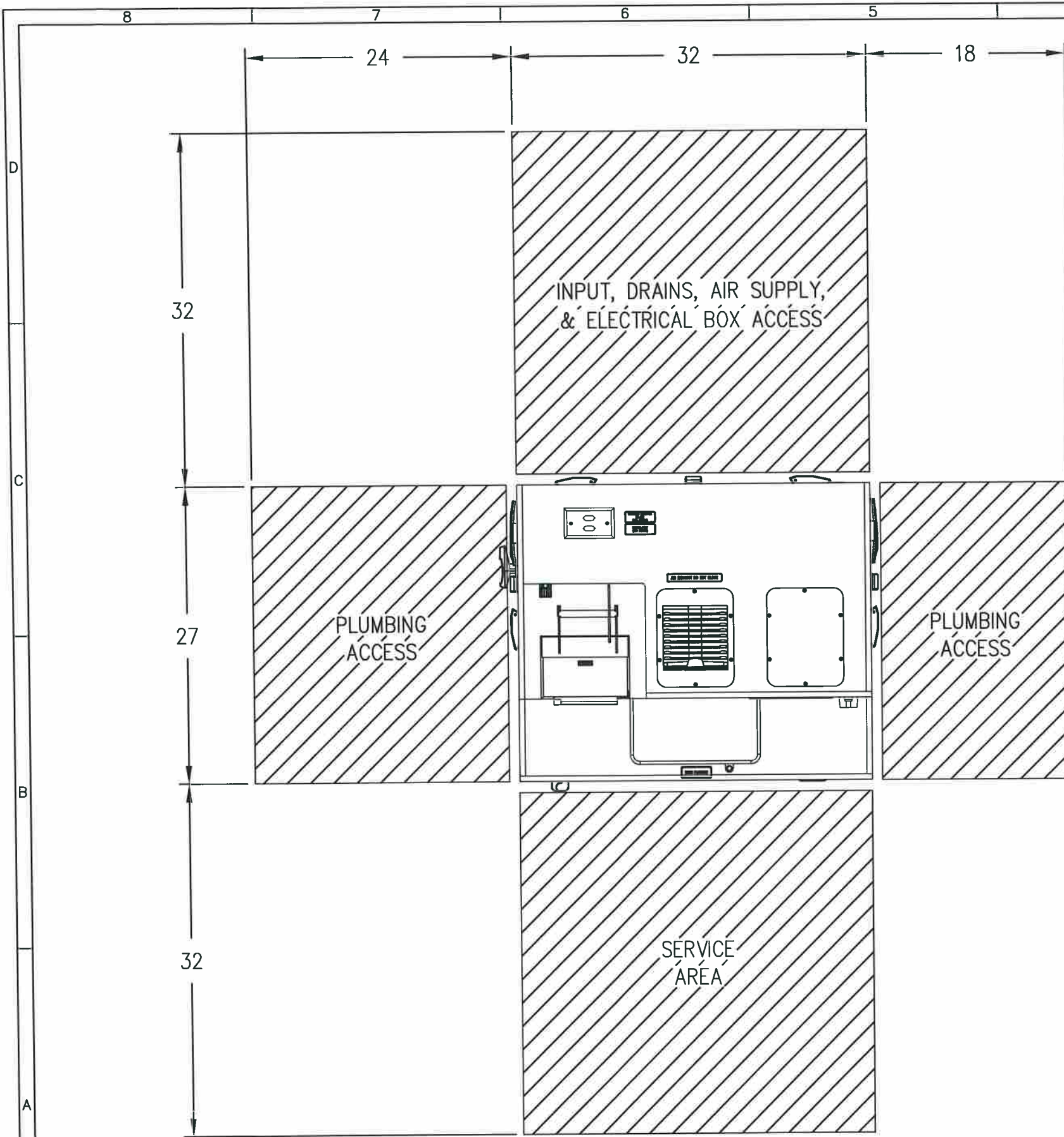
DEMETER DISPENSE SYSTEM FOOTPRINT TOP VIEW
