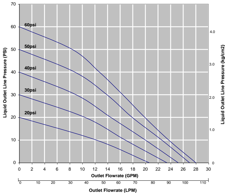
AT300HD Head Pressure Line Chart
