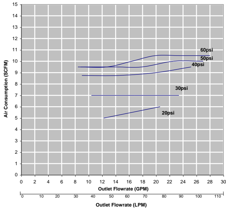
AT300HD Air Consumption Line Chart
