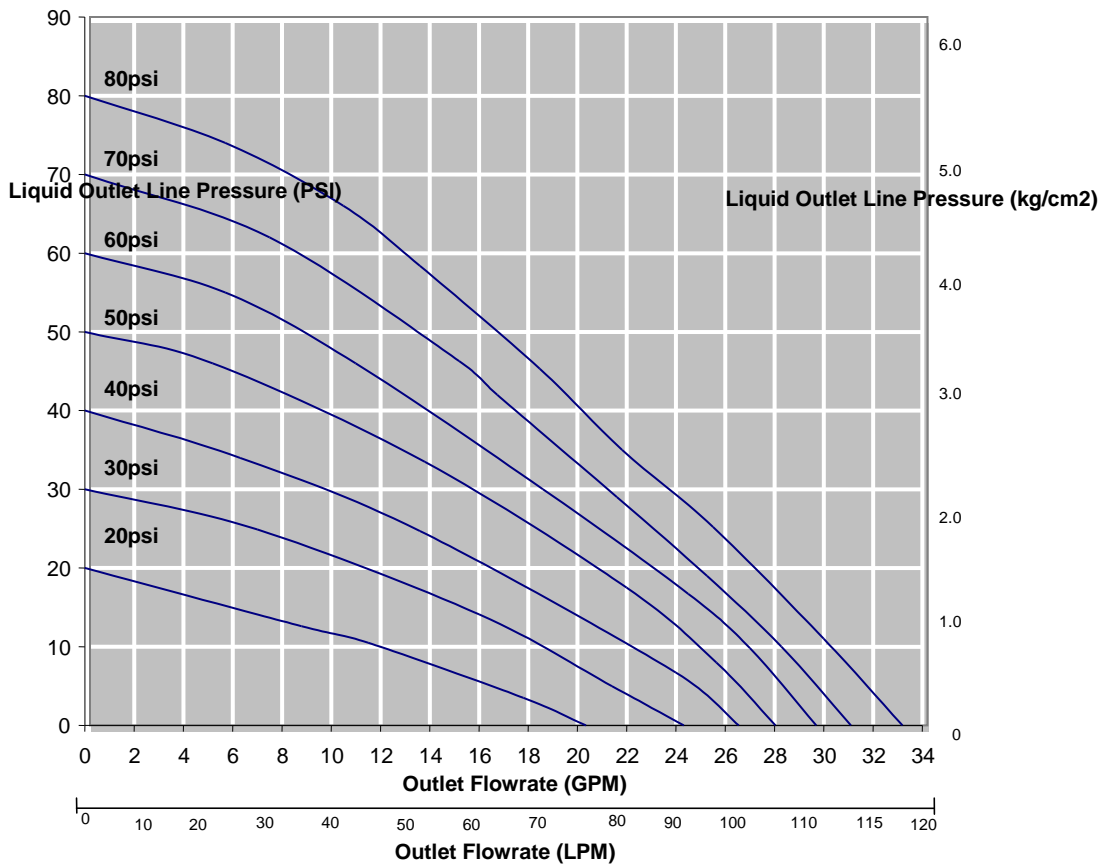
PL120 Head Pressure Line Chart
