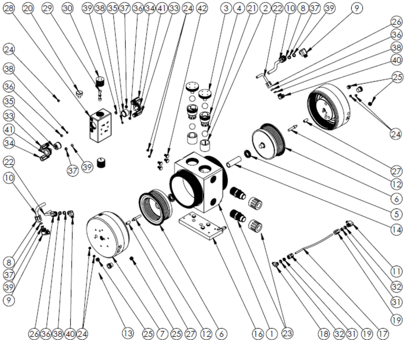
PL120 Bill of Materials
